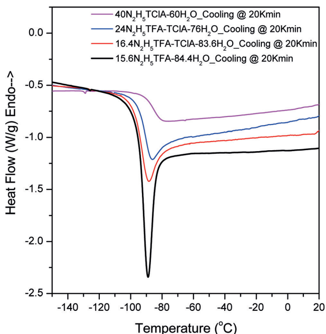
Figure 2. DSC downscans at 20 \text{ K min}^{-1} of solutions of inorganic salts with large \text{N}_2\text{H}_5^+ cations and trihaloacetate anions or their mixtures, showing normal glass transition at lower (60 mol %) water content and “spike” anomalies at high water contents.
